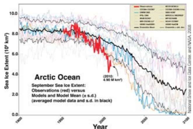
Fig.22 Arctic September sea ice extent from observations (red line) and 13 IPCC AR4 climate models (updated from Stroeve et al. 2007).
