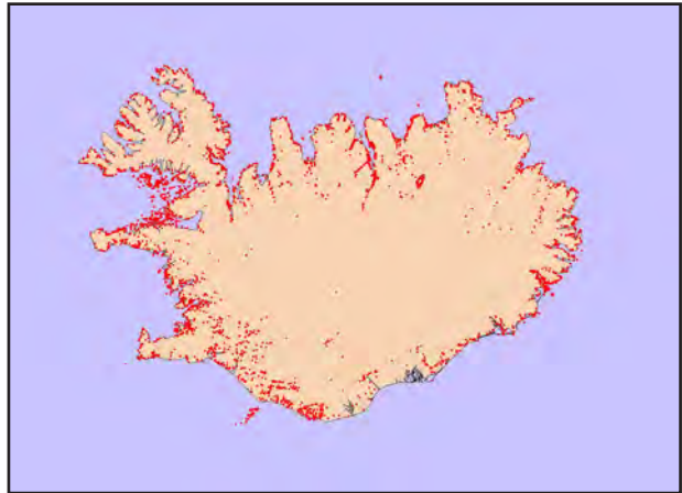
Fig. 1. The distribution of seabird colonies in Iceland. The map shows around 3500 colony sites but it is estimated that individual sites may be as many as 4500. From Bakken et al. (2006).
